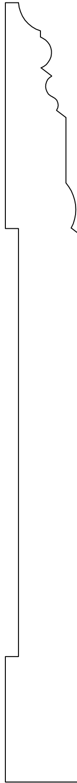
CST 4003 1\frac{3}{16} \times 8\frac{1}{4}
